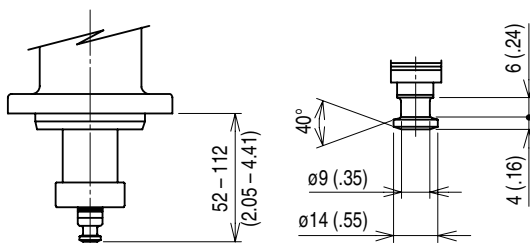
STEM BUTTON DETAIL
