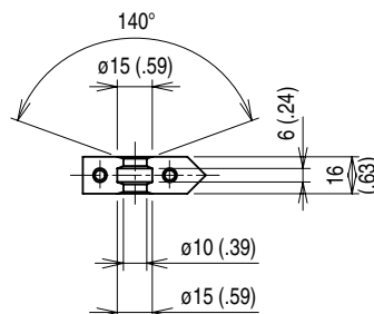
INDICATOR DETAIL
