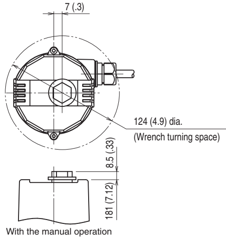
YOKE CONNECTION
