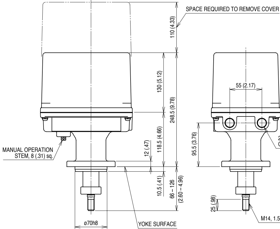
YOKE CONNECTION
