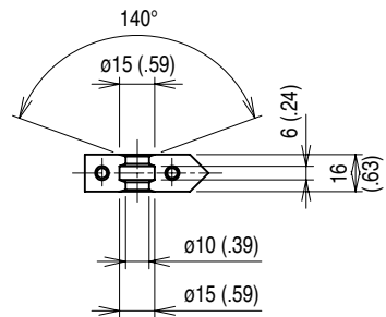
INDICATOR DETAIL
